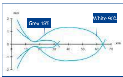
Detection area
