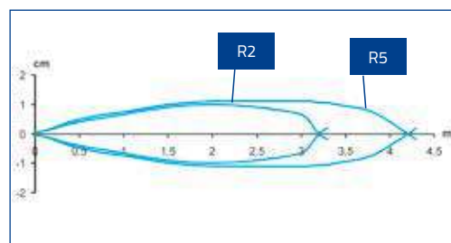
Detection area
