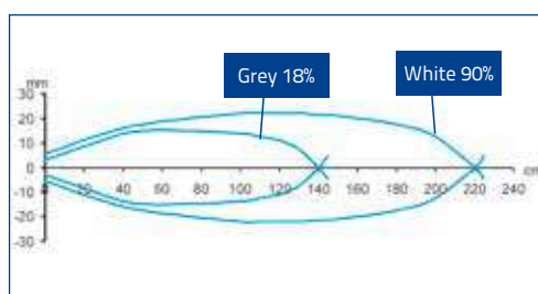
Detection area
