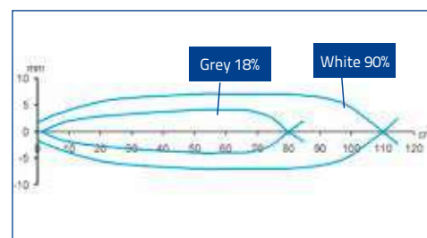
Detection area
